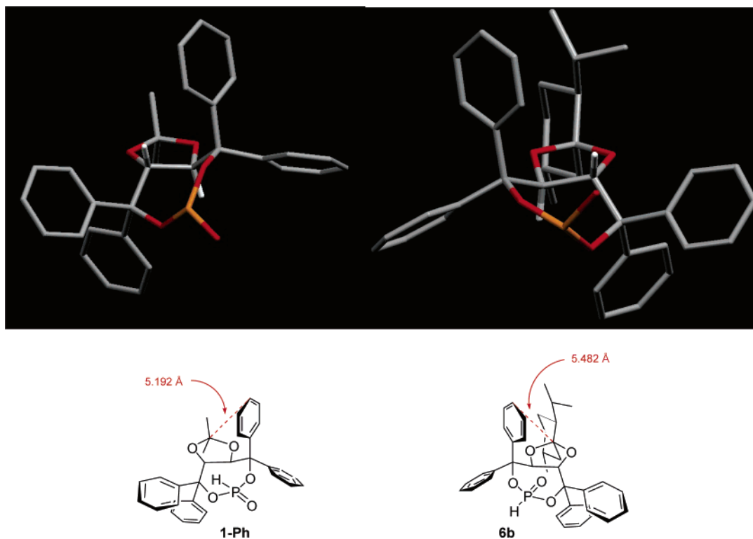
Figure 2. X-ray structures of phosphites 1-Ph and 6b .
