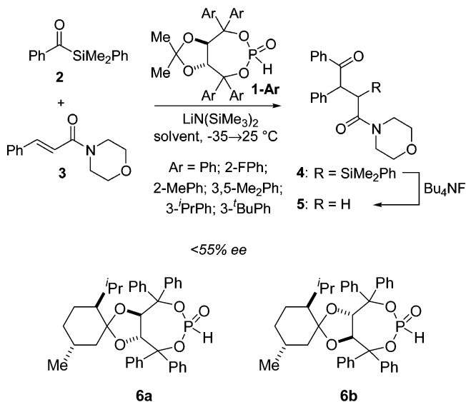
Figure 1. TADDOL-phosphites containing the l -menthone ketal.
